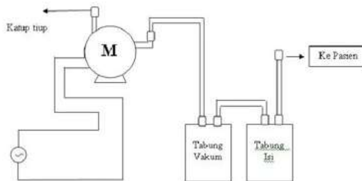
Gambar 2.3 Rangkaian Suction [4]
