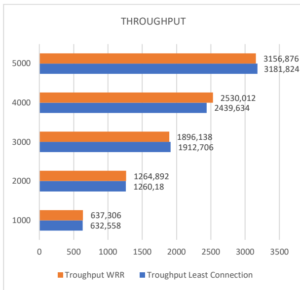
GAMBAR 9 THROUGHPUT
