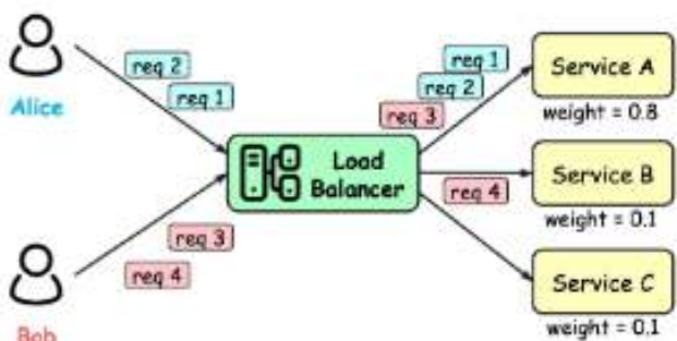
GAMBAR 2 WEIGHTED ROUND ROBIN [5]
