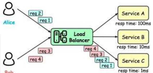
GAMBAR 4 LEAST RESPONSE TIME [5]
