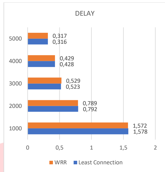
GAMBAR 10 DELAY
