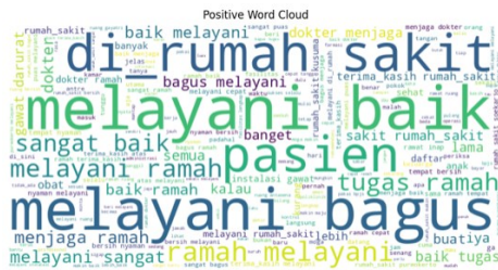
GAMBAR 6 (WORDCLOUD POSITIF)
