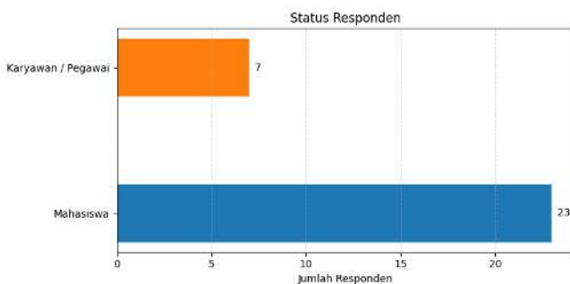
GAMBAR 7 Status Responden
