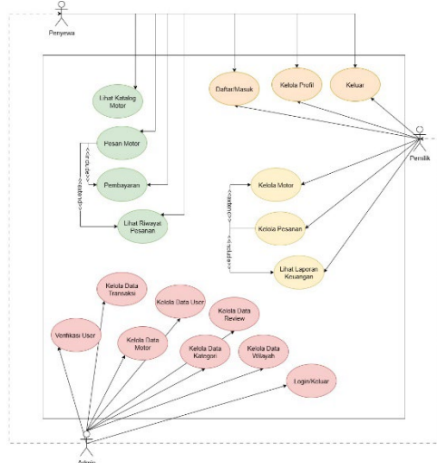
GAMBAR 2 Usecase Diagram
