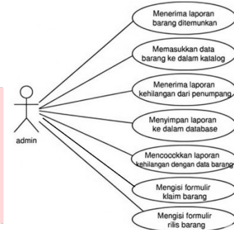
GAMBAR 4 Usecase Diagram
