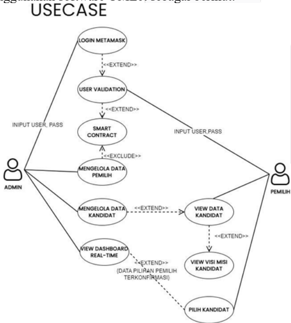
GAMBAR 2 Use Case E-Voting
