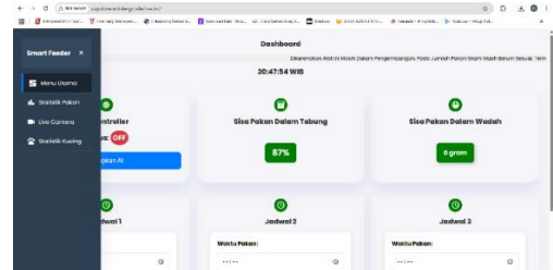
Gambar 9. Tampilan Website
