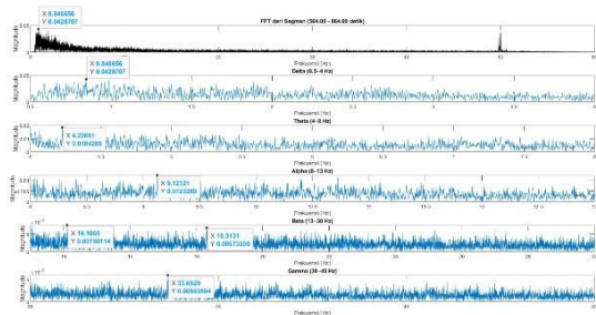
GAMBAR 36 (Magnitude Stimulus Audio)
