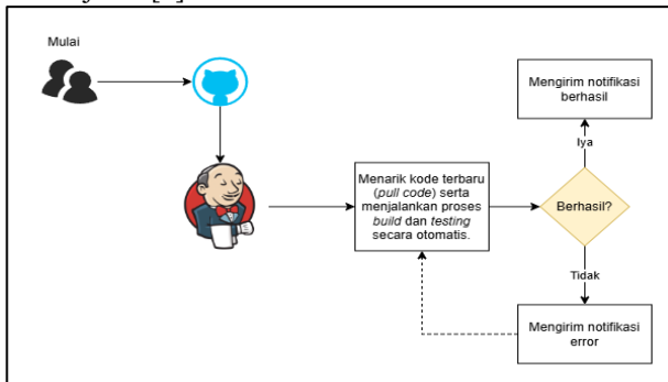
Gambar 2.2 Arsitektur Continuous Integration (CI)
