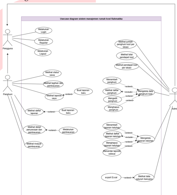
Gambar 4.1 Usecase Diagram
