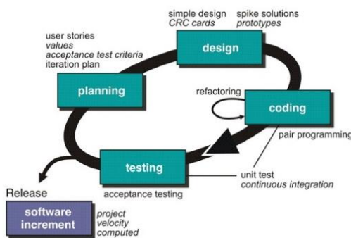
GAMBAR 2 Extreme Programming
