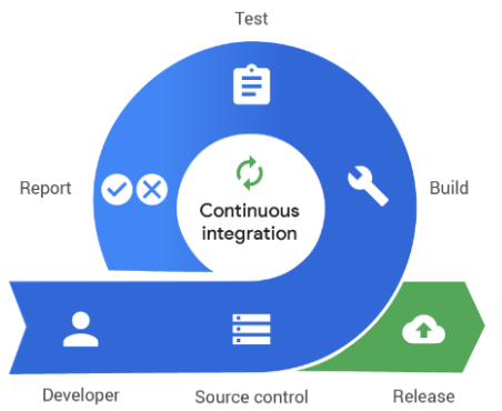
GAMBAR 1 Continuous Integration
