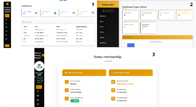
GAMBAR 4 Tampilan Dashboard
