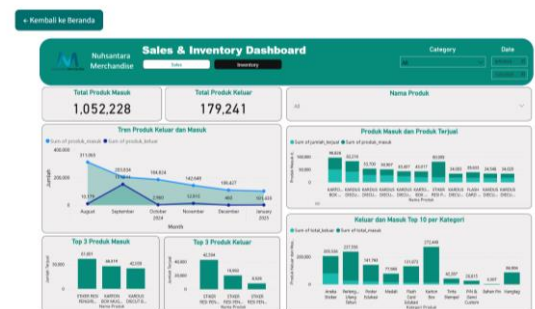
Gambar 9 (Inventory)
