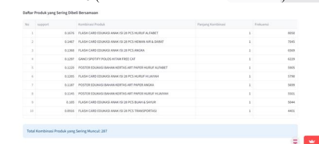
Gambar 14 (Frequent itemsets)
