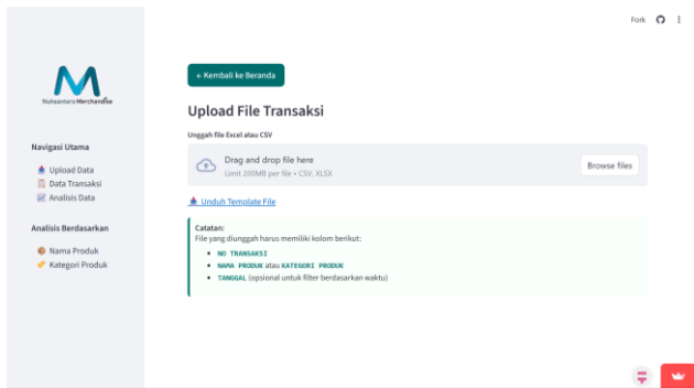
Gambar 11 (Upload File)
