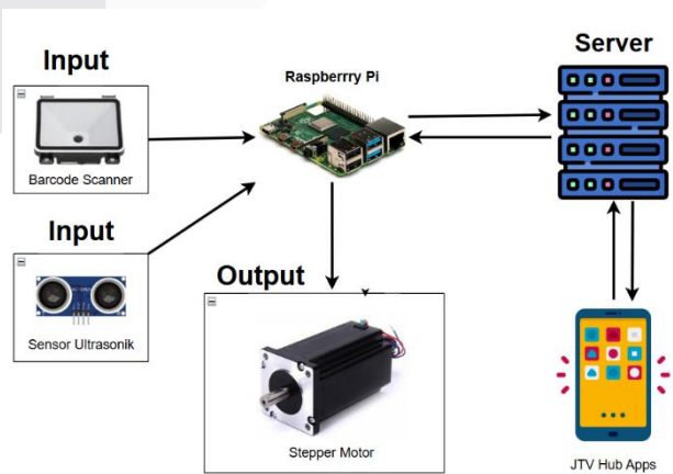
Gambar 2 Blok Diagram
