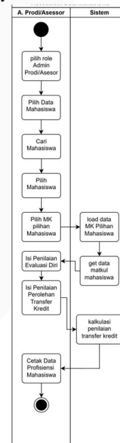
GAMBAR 4 Activity Proses Asesmen
