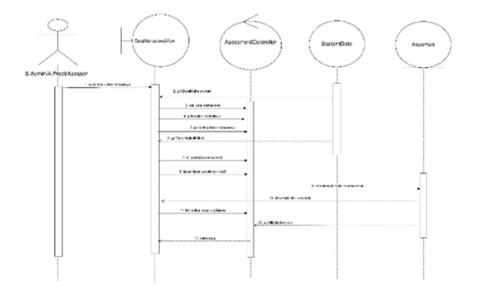
GAMBAR 5 Sequence Diagram Proses Asesmen
