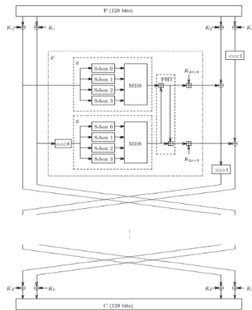
Gambar 1. Blok Diagram Twofish
