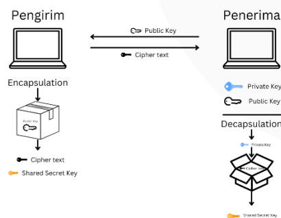
Gambar 2. Encapsulation Mechanism
