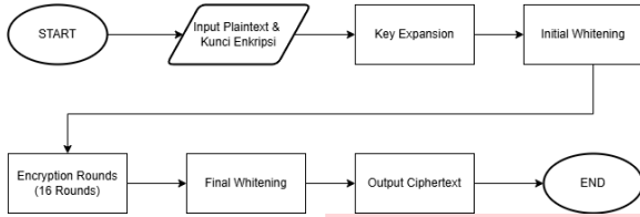
Gambar 5. Enkripsi Twofish
