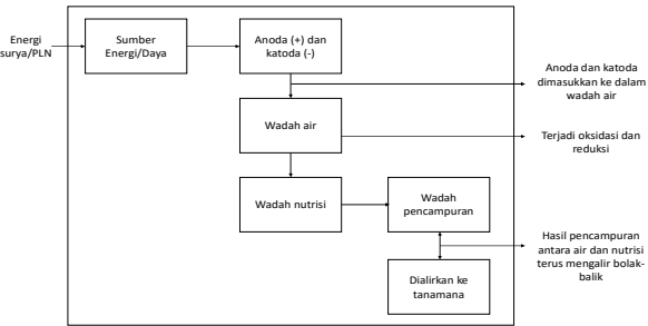
GAMBAR 4 (Diagram Blok Level 1)
