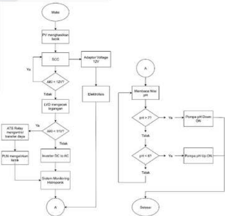
GAMBAR 6 (Flowchart System)
