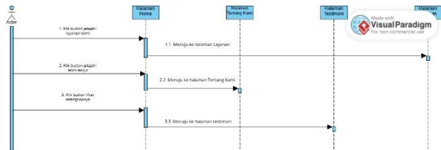
Gambar 2 Sequence Diagram pelanggan home
