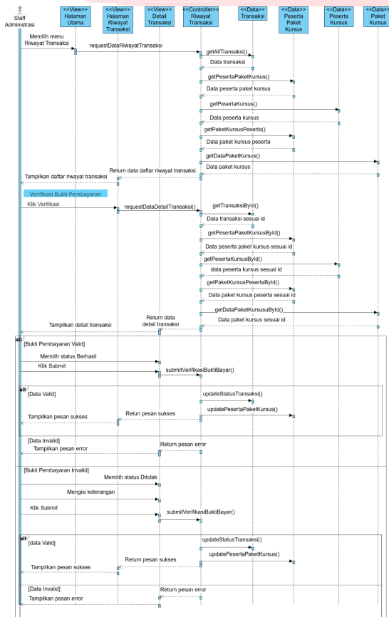
Gambar IV. 3 Sequence Diagram Kelola Riwayat Transaksi
