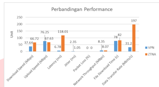
Gambar 7 Perbandingan Performance
