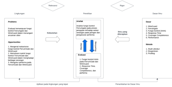
Gambar 1 Model Konseptual
