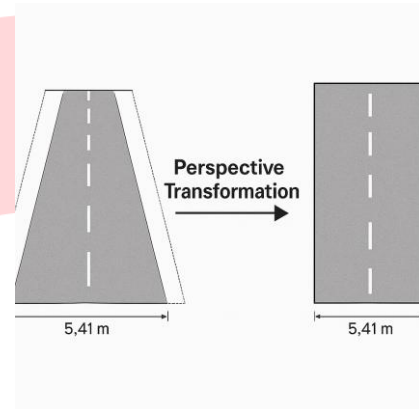
GAMBAR 2 (Perspective Transformation)
