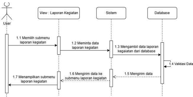
Gambar IV-4 Sequence Diagram
