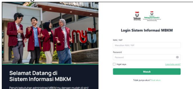
Gambar IV-5 Login Interface
