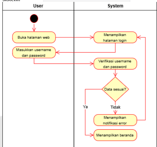
Gambar IV-3 Activity Diagram
