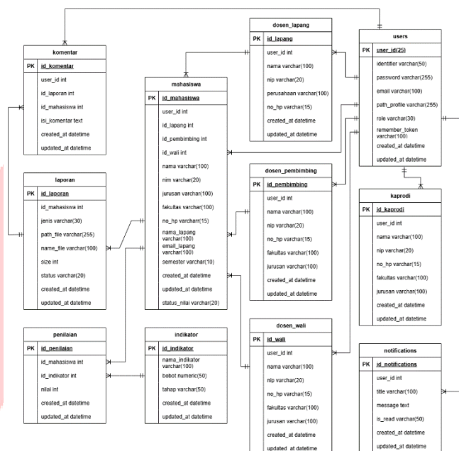
Gambar IV-2 Entity Relationship Diagram
