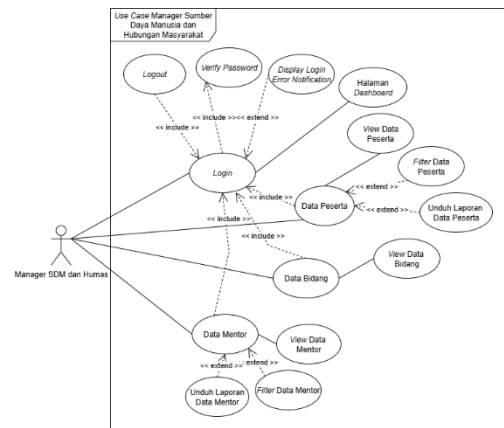
GAMBAR 3 Use Case Diagram Manager SDM dan Humas
