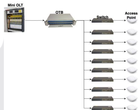
Gambar 2 Desain sistem jaringan Fiber To The Building
