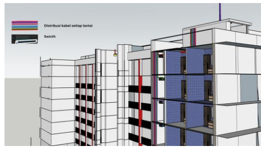
Gambar 4 Drafting jalur fiber optic
