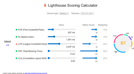
Gambar 11 Skor Google Lighthouse
