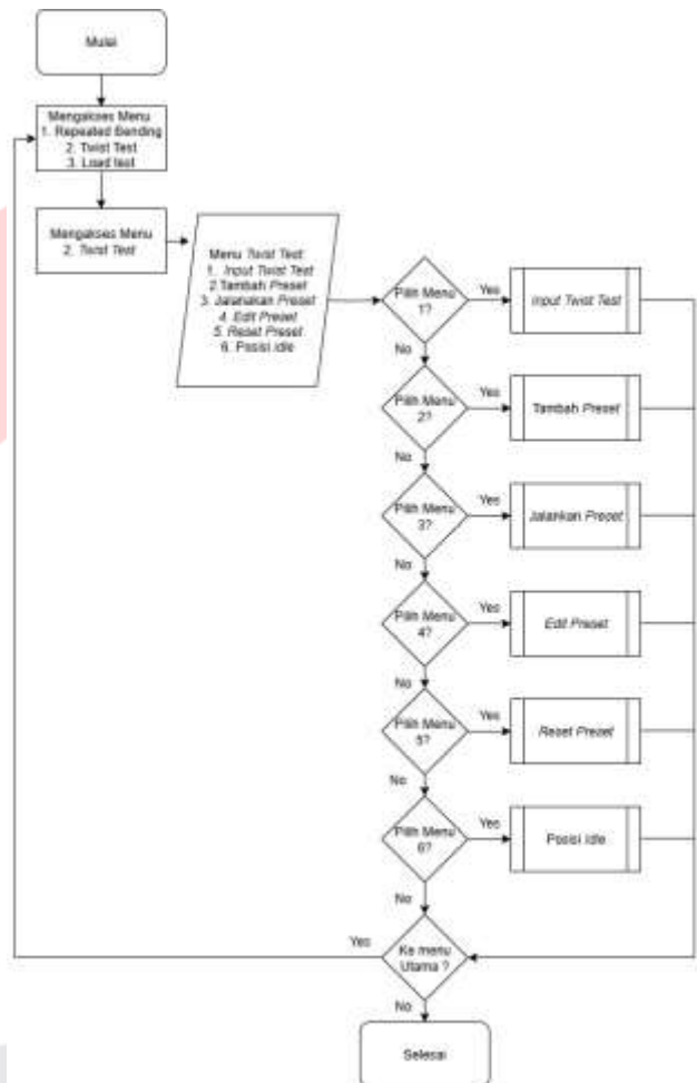
Gambar 4 Flowchart Alur Pengujian Twist
