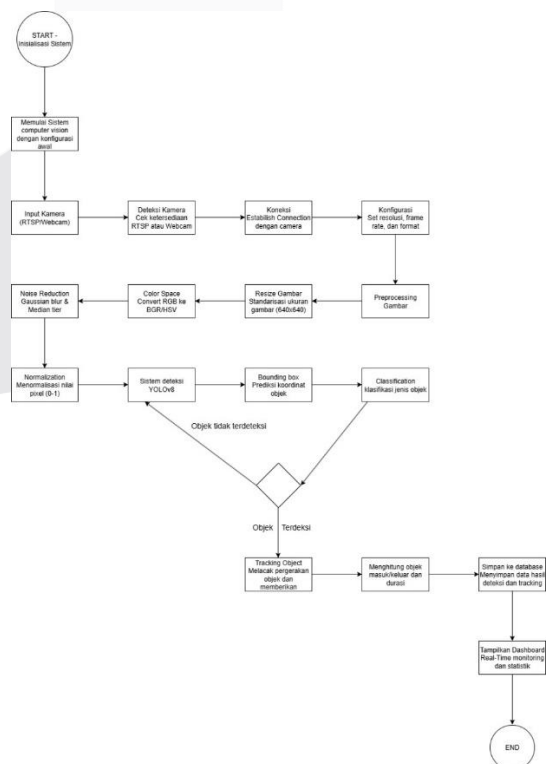
Gambar 2 Diagram Alir Sistem People Counter System
