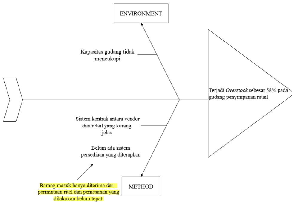
Gambar I. 4. Fishbone Diagram
