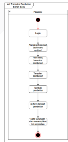
GAMBAR 10 Activity Diagram Pembelian Bahan Baku
