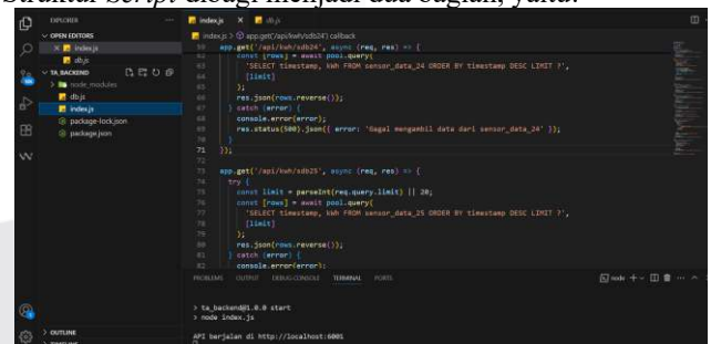
Gambar 4.1 Script Backend
