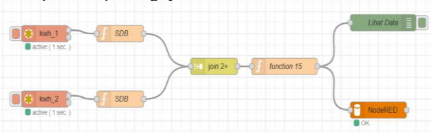
Gambar 4. 3 Flow SDB 1
