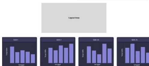
Gambar 3.4 Mockup Dashboard
