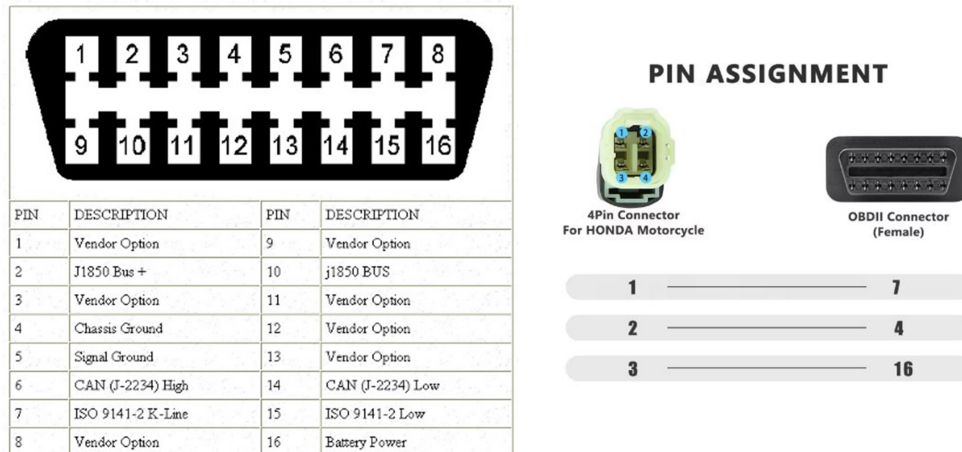
Gambar 2. 2 OBD-II Connector Pin
