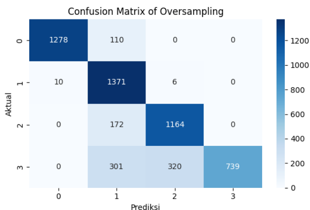
GAMBAR 5 (CONFUSION MATRIX SMOTE)
