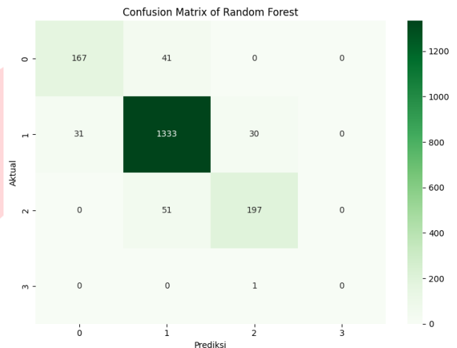
GAMBAR 4 (CONFUSION MATRIX RF)
