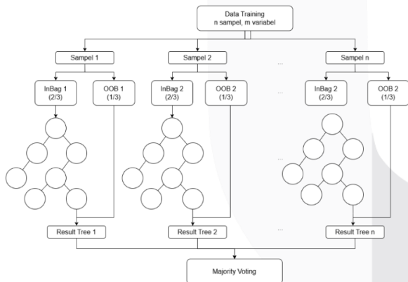
GAMBAR 1 (CARA KERJA RANDOM FOREST [15])
