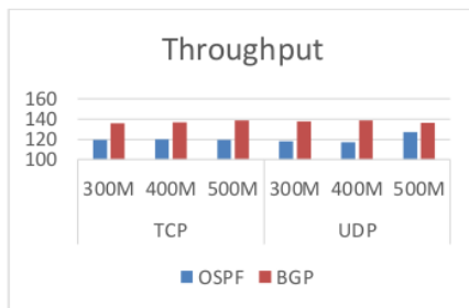
Gambar 4. 3 grafik throghput
