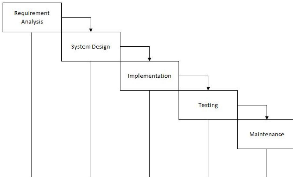
Gambar 1.1 Metode Waterfall
