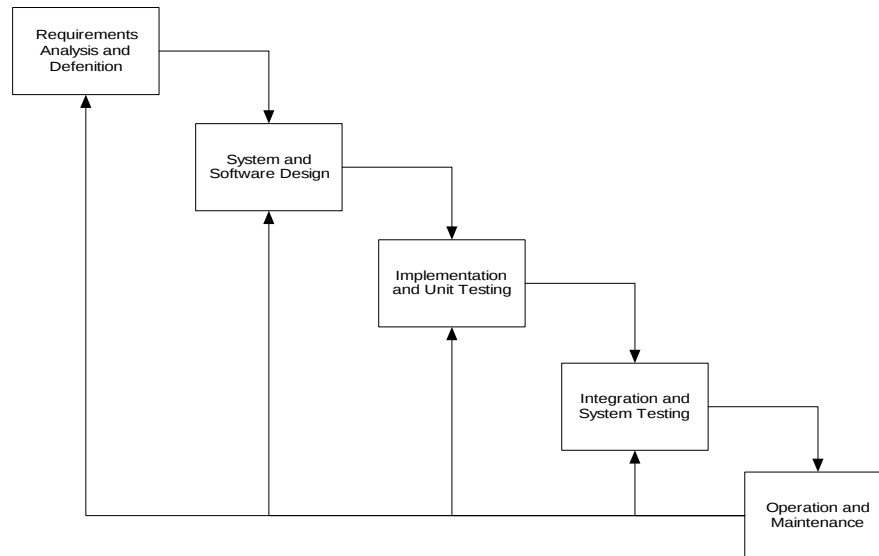
Gambar 1-1 Model Waterfall [1]
