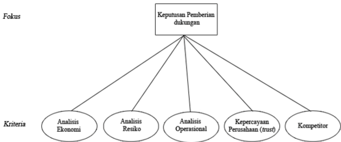
Gambar 1-1 Criteria Tree
