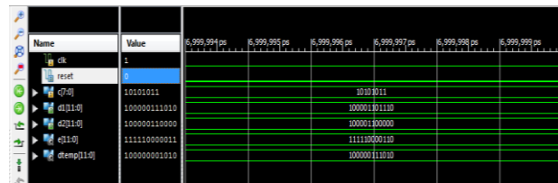
Gambar 4.11 Test bench Loop Filter
